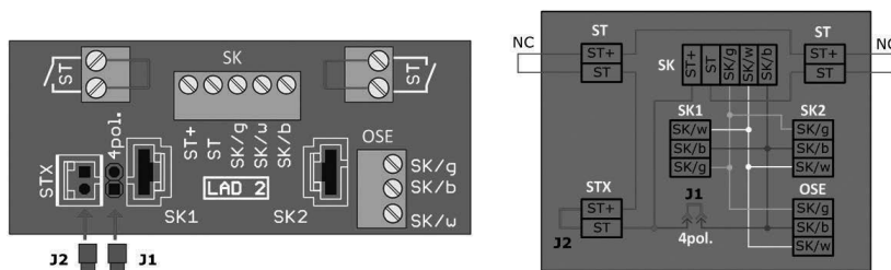
Figure 3 – Switching module
